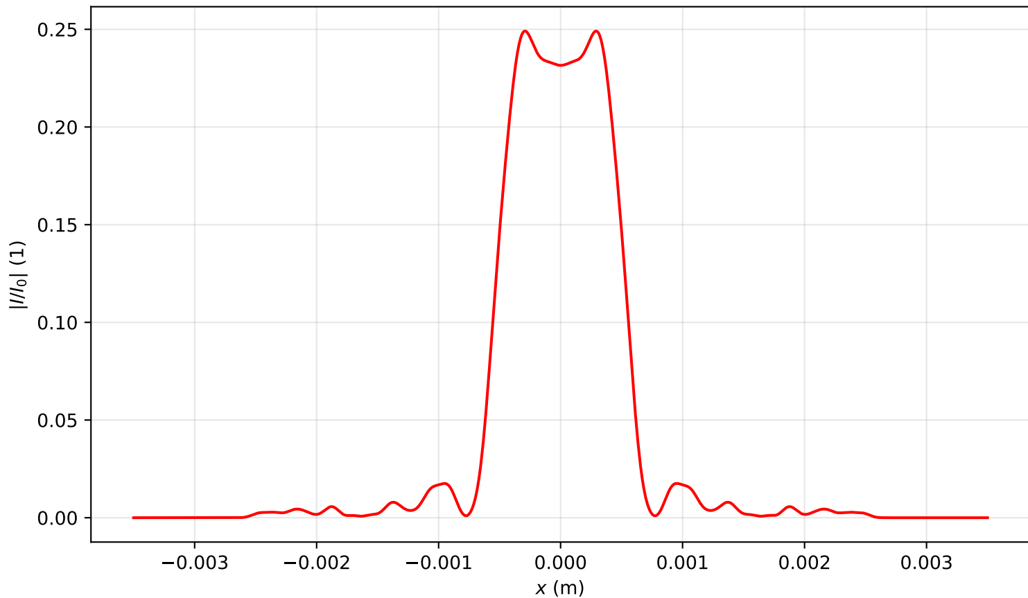
Intensity profile I(x, y = 0, z = 1.751)/I_0 , P_{in}=4.0P_{cr} , artificial time
